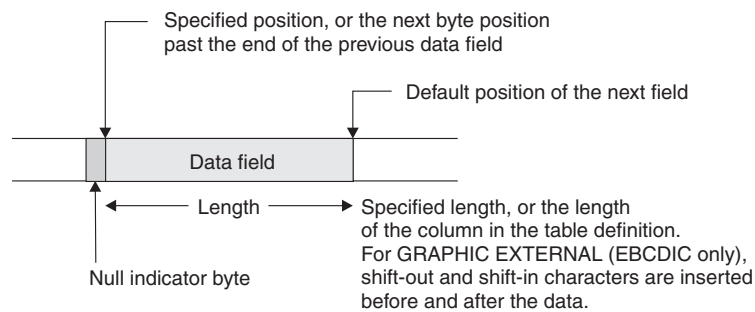
Figure 99. Layout of a nullable fixed-length field
