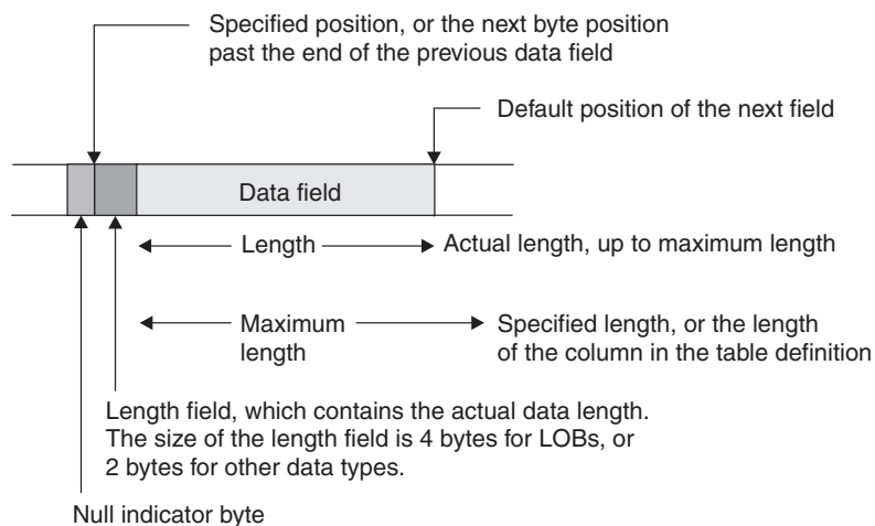
Figure 102. Layout of a nullable varying-length field with the NOPAD option
