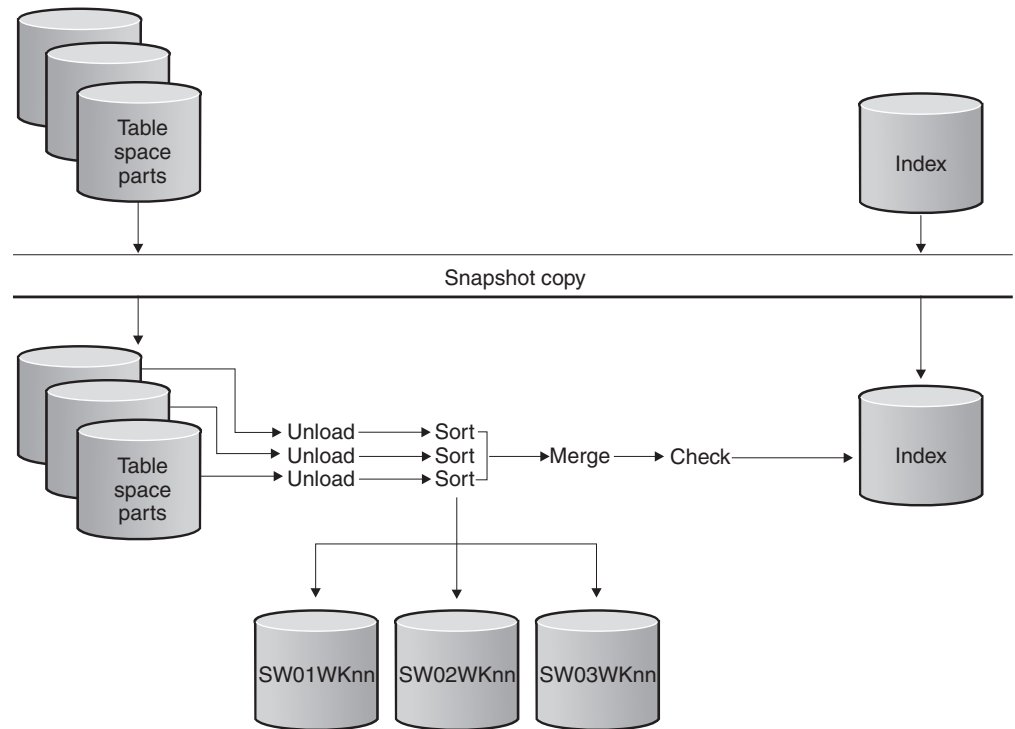
Figure 11. Parallel index check for a partitioned table space with a single nonpartitioned secondary index
