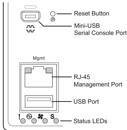
Figure 3. G8296 rear panel
