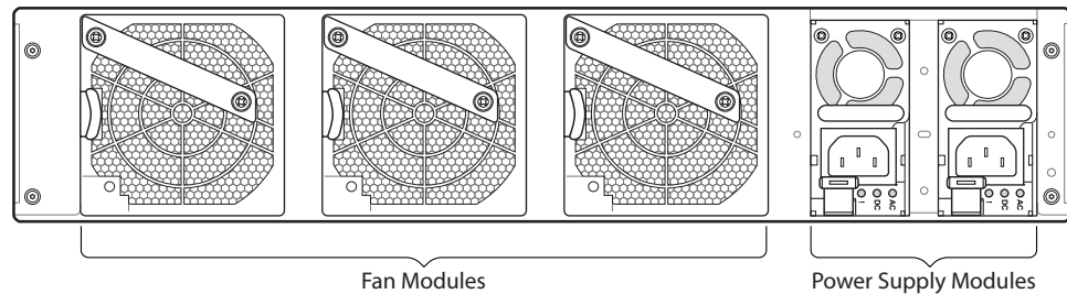
Figure 3. G8296 rear panel
