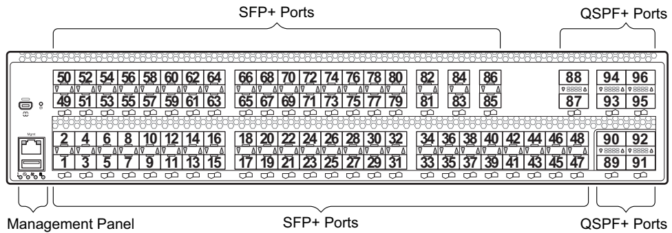
Figure 2. G8296 management panel detail
