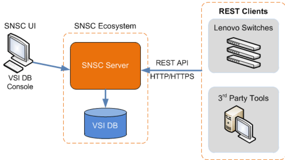
Figure 88. VSI database
