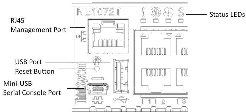
Figure 3. NE1072T rear panel
