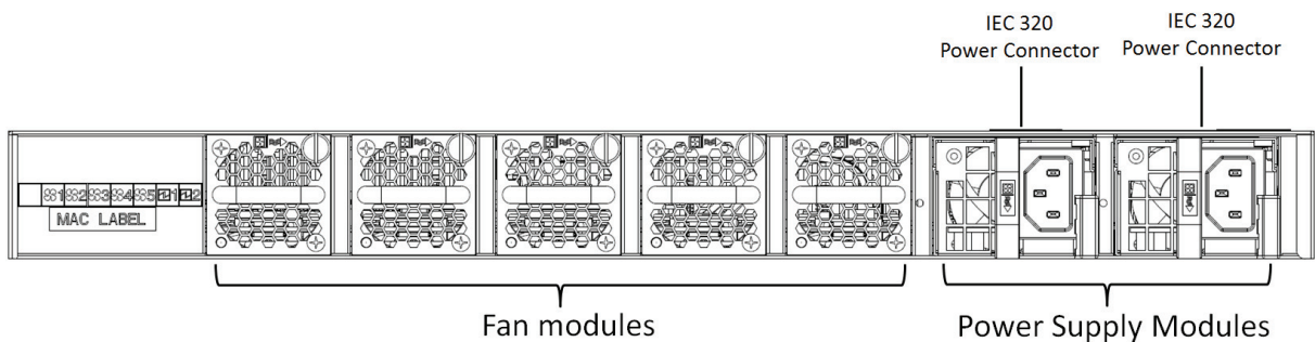
Figure 3. NE1072T rear panel
